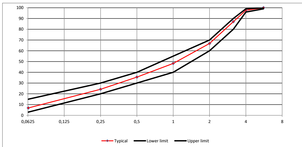
Indicating aggregate grading curve (w/w%)
